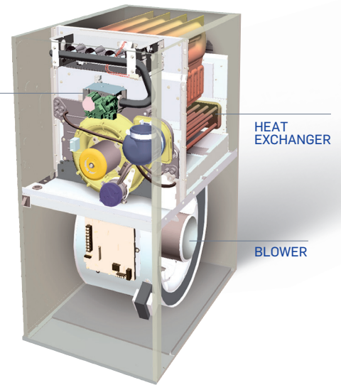
PERFORMANCE 96 GAS FURNACE
